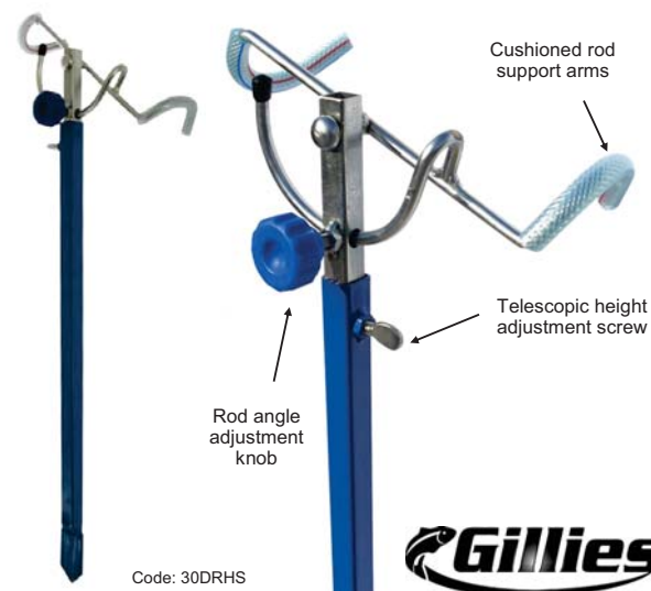
Spring loaded cushioned rests
